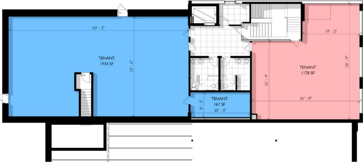
3 THIRD FLOOR Copy 1 1" = 10'-0"
