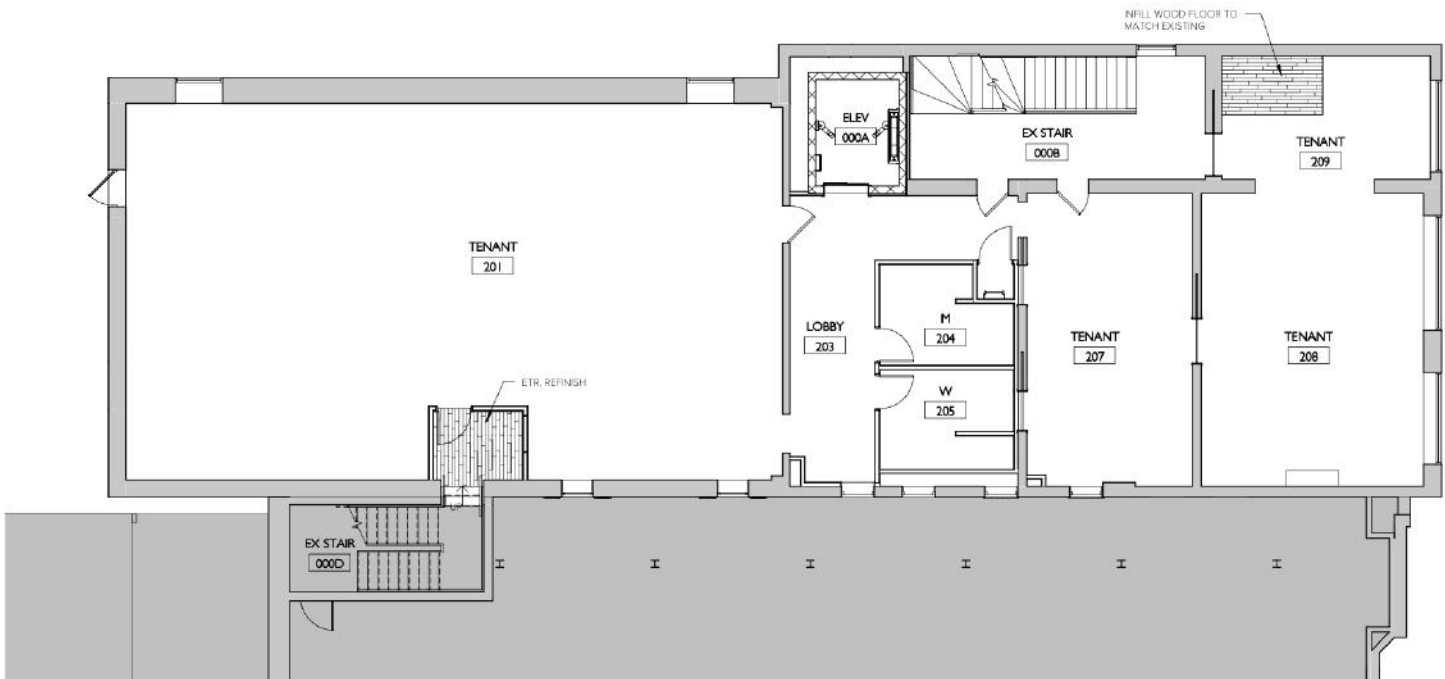
SECOND FLOOR FINISH PLAN
